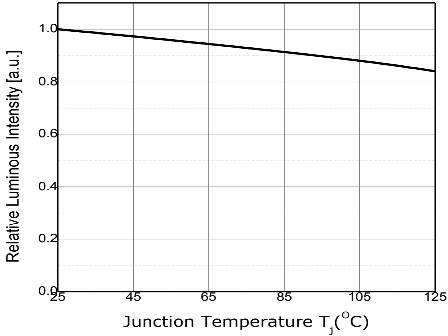
Fig 6. Junction Temperature vs. Relative Luminous Intensity, I_F=65\text{mA}
