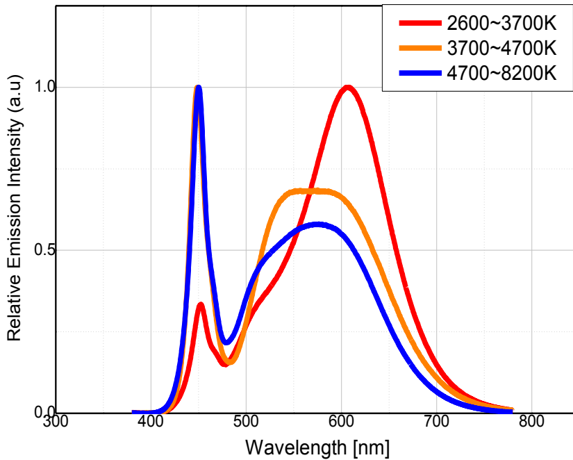
Fig 1. Color Spectrum, T_j = 25^\circ\text{C} , I_F = 65\text{mA}
