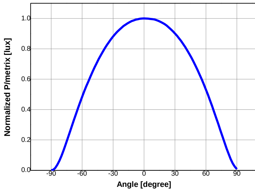
Fig 2. Radiant pattern, I_F = 20\text{mA}
