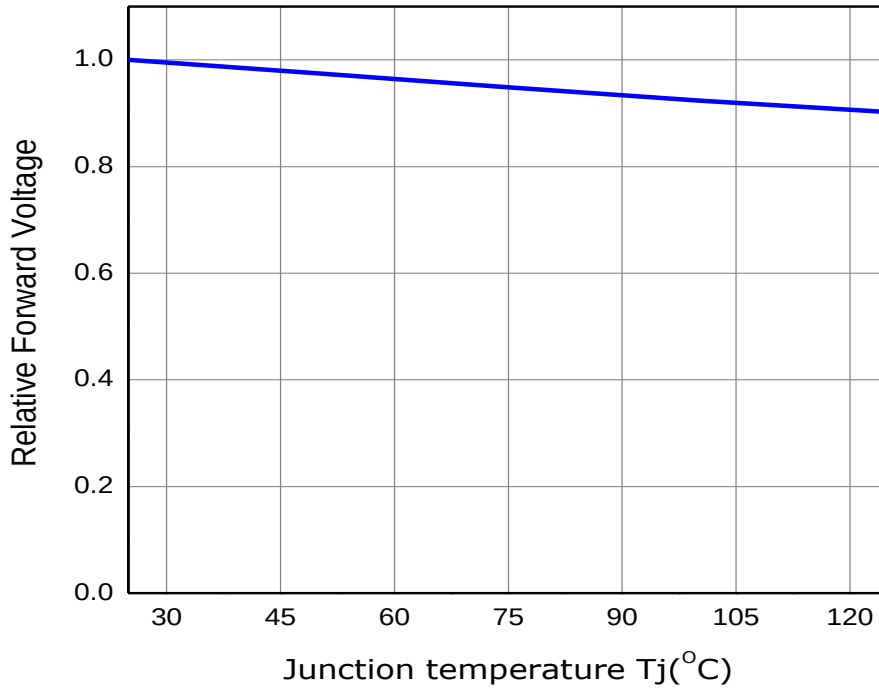
Fig 6. Relative Forward Voltage vs. Junction Temperature, I_F=20\text{mA}
