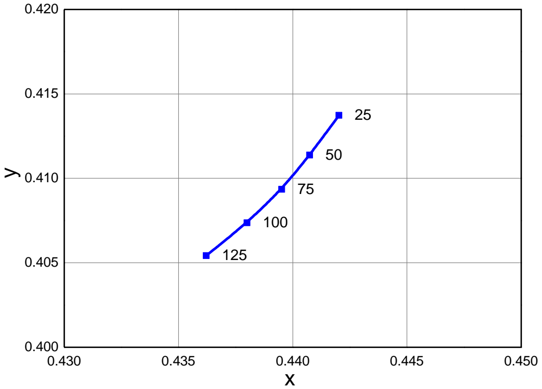
Fig 8. Junction Temp. vs. Chromaticity Coordinate , I_F=20mA
