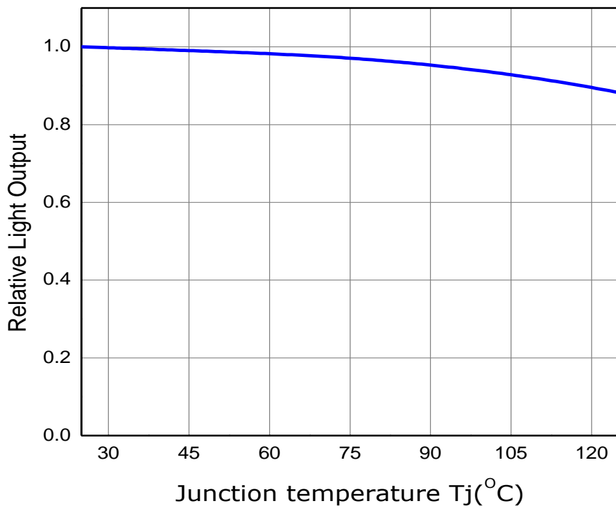
Fig 7. Junction Temp. vs. Relative Light Output, I_F=20mA
